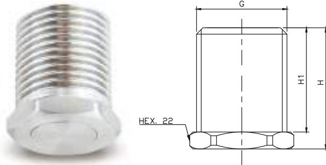
KS1 Series : 3/4" & 1/2"
