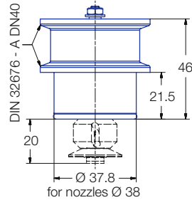
Tri-Clamp
