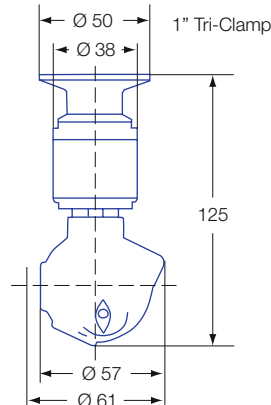
1" Tri-Clamp
