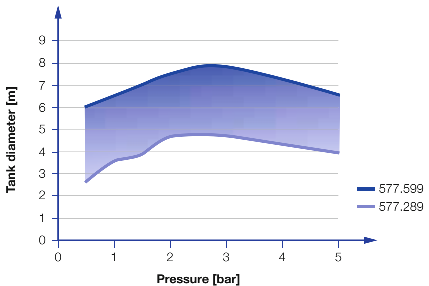
Overview of the tank diameter, depending upon the pressure of series 577 / 579
